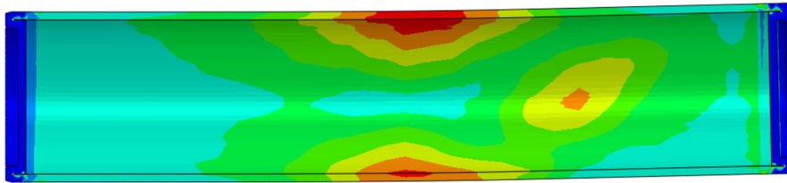
Calc. 1. Reference case. 5 cm shear. Max peeq 0.16
