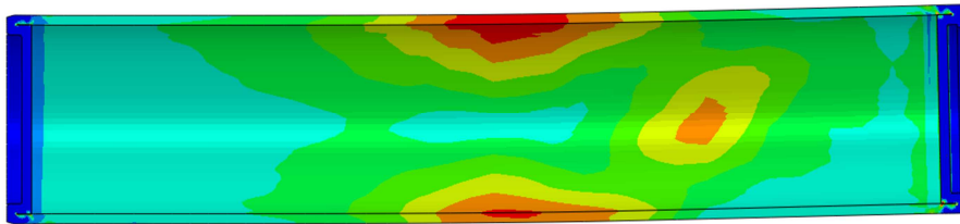
Calc. 2. Brittle. 5 cm shear. Max peeq 0.16
