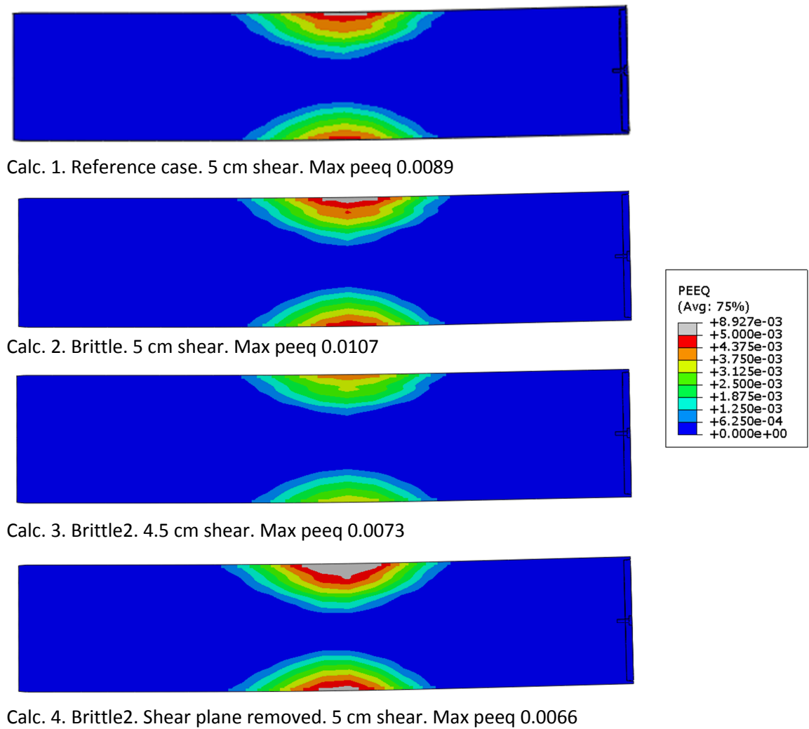
Figure 9. Plastic strain (peeq) in the insert.
