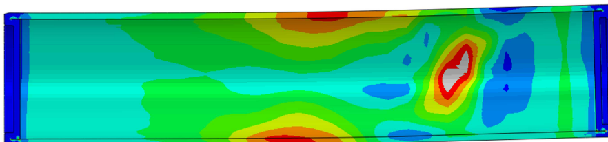
Calc. 4. Brittle2. Shear plane removed. 5 cm shear. Max peeq 0.15
