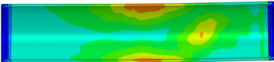
Calc. 3. Brittle2. 4.5 cm shear. Max peeq 0.16
