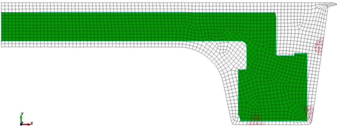
Figure 3-17. Location of circular cracks in workpiece after the closed die forging, step 4, with inherited stresses and effective plastic strains from step 3. Note that the workpiece is at room temperature.
