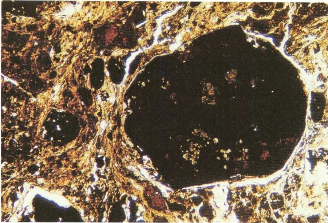
PLATE 3. Borehole MF10 (sample MF10-1-12); representative photomicrograph of the Th-REE ore consisting of magnetite nodules oxidized to variable degrees and embedded in a fine-grained matrix. Inclusions of primary bastnaesite occur in the large magnetite nodule (mag. 25x).
