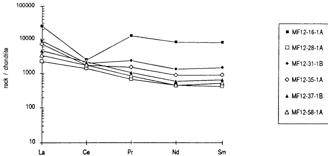
Figure 16. Borehole MF12: LREE normalized to ordinary chondrite (analysis by ICPOES; for normalization factors, see Table IV).
