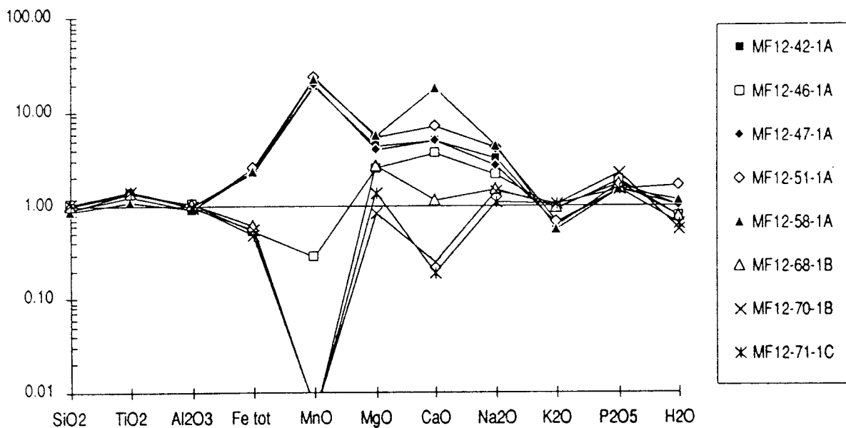
Figure 10. Borehole MF12: major elements for the reduced hydrothermally altered phonolites normalized to the average for reduced hydrothermally altered phonolites of the Osamu Utsumi mine (data from Waber et al., this report series; Rep. 2).
