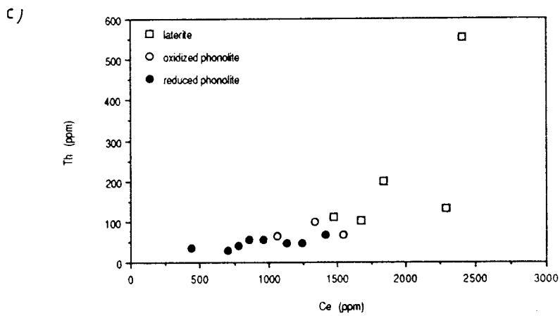
Figure 18. Borehole MF12: binary plot of: a) lanthanum versus cerium, b) lanthanum versus neodymium, and c) thorium versus cerium, for the different rock units (analysis by XRF).
