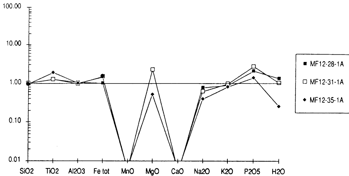
Figure 14. Borehole MF12: major element contents of the oxidized hydrothermally altered phonolites normalized to the average of the oxidized hydrothermally altered phonolites from the Osamu Utsumi mine (data from Waber et al., this report series; Rep. 2).
