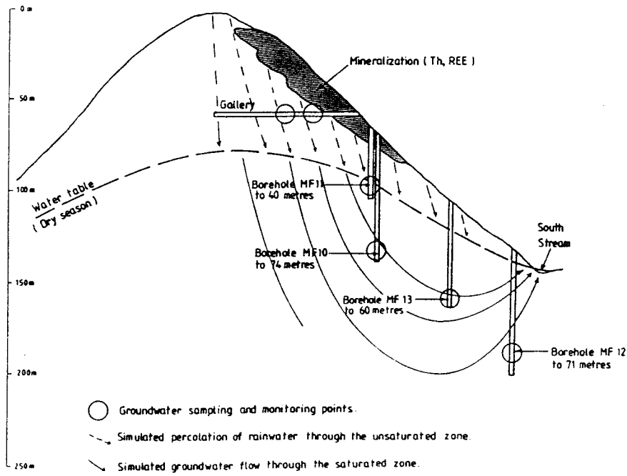
Figure 4. Location of boreholes MF10 to MF13 at Morro do Ferro in relation to the mineralization and the dry season water table.
