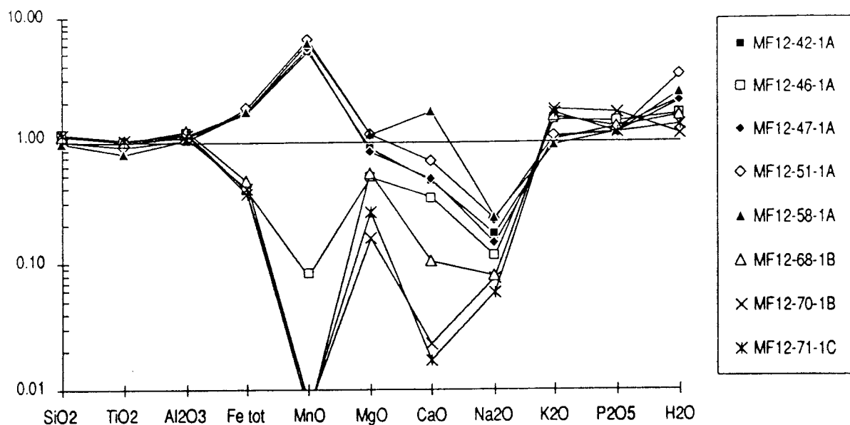
Figure 9. Borehole MF12: major elements for the reduced hydrothermally altered phonolites normalized to the average for regional phonolites (data from Schorscher and Shea, this report series; Rep. 1).
