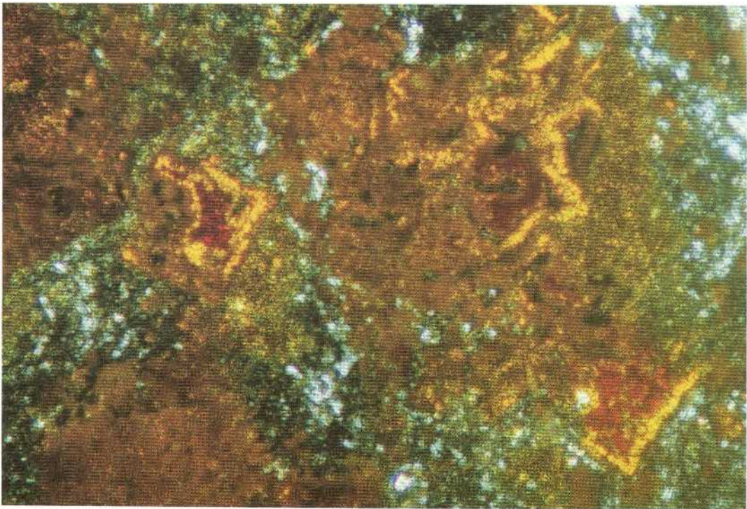
PLATE 4. Borehole MF10 (sample MF10-4-1A); photomicrograph showing hematite (red), goethite (yellow) and poorly crystalline ferric oxides in close association, replacing idiomorphic magnetite. Matrix consists of kaolinite and gibbsite (mag. 25x).
