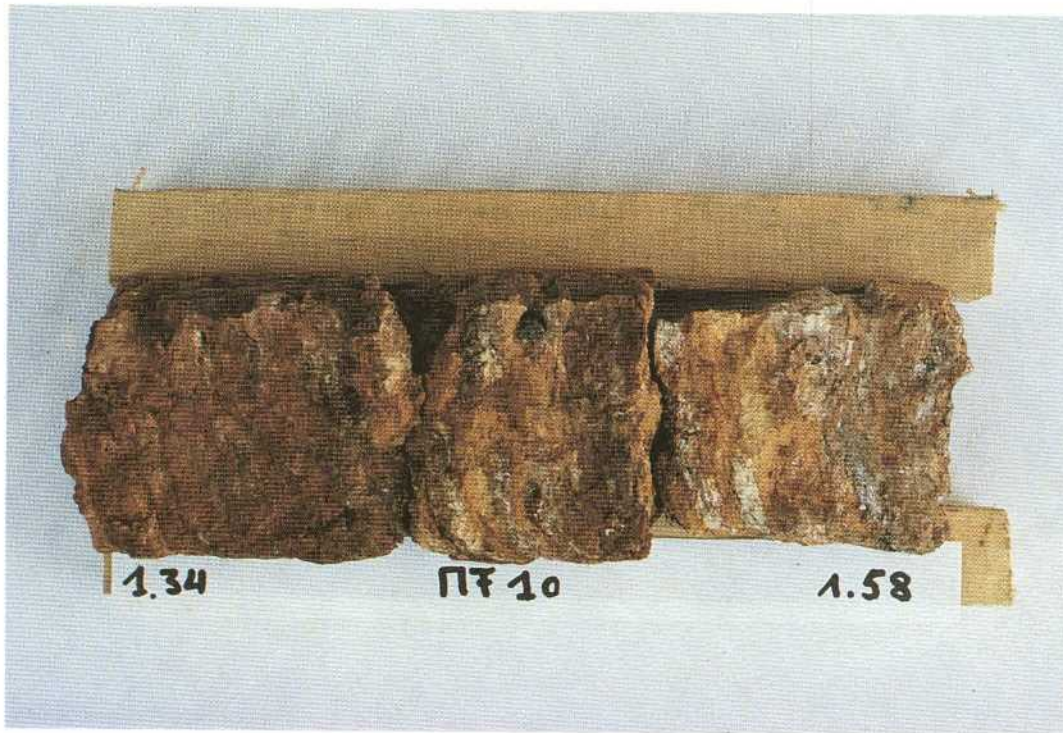
PLATE 1. Borehole MF10; typical core section of the Th-REE ore body with magnetite nodules.
