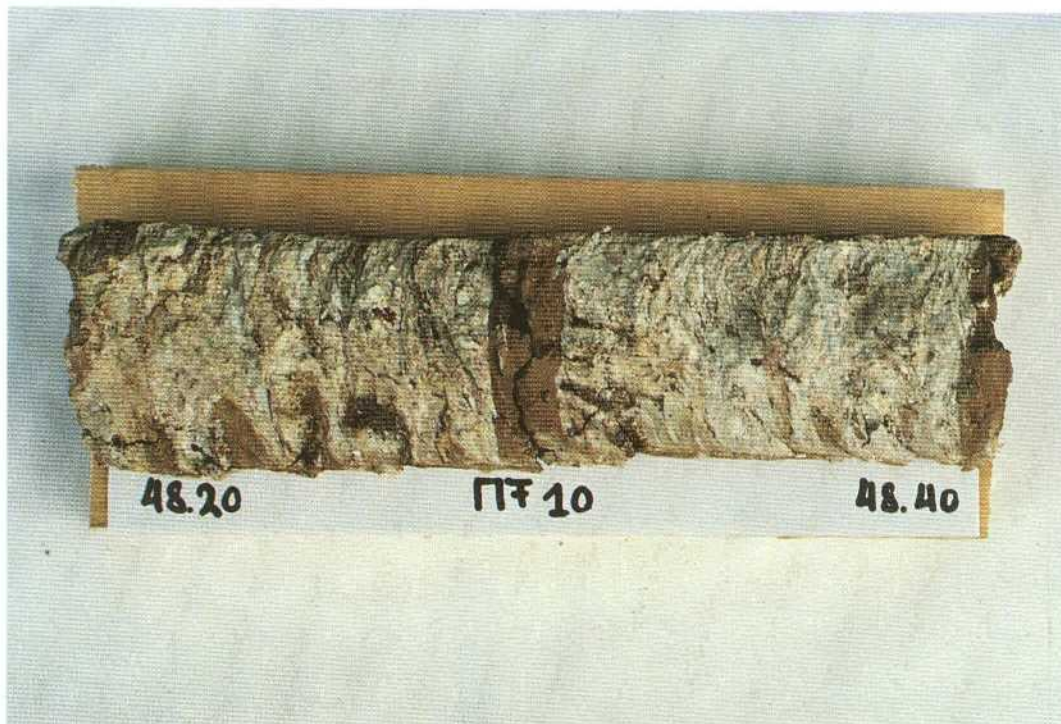
PLATE 2. Borehole MF10; typical core section of the carbonatitic host rock (completely weathered) below the ore body.
