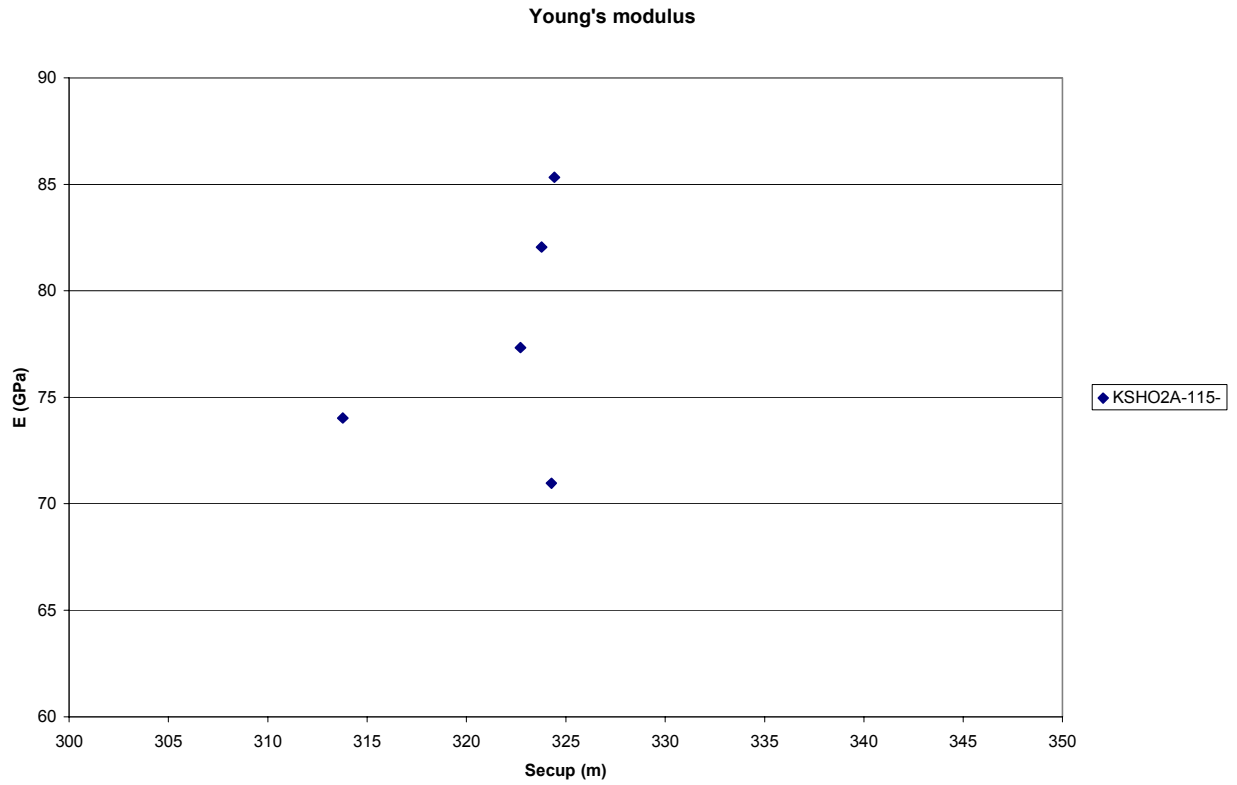
Figure 5-3. Tangent Young's modulus versus depth at which the samples are taken in the borehole.
