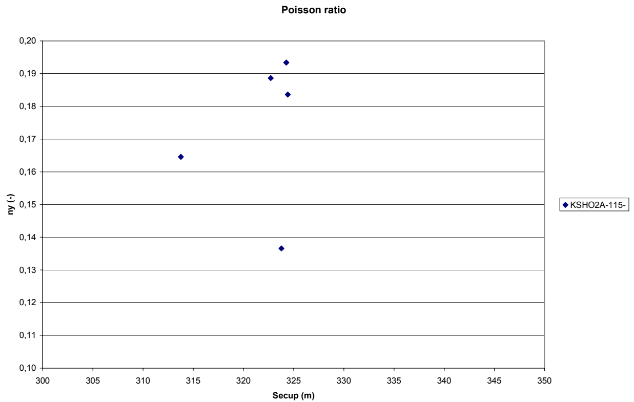
Figure 5-4. Tangent Poisson ratio versus depth at which the samples are taken in the borehole.
