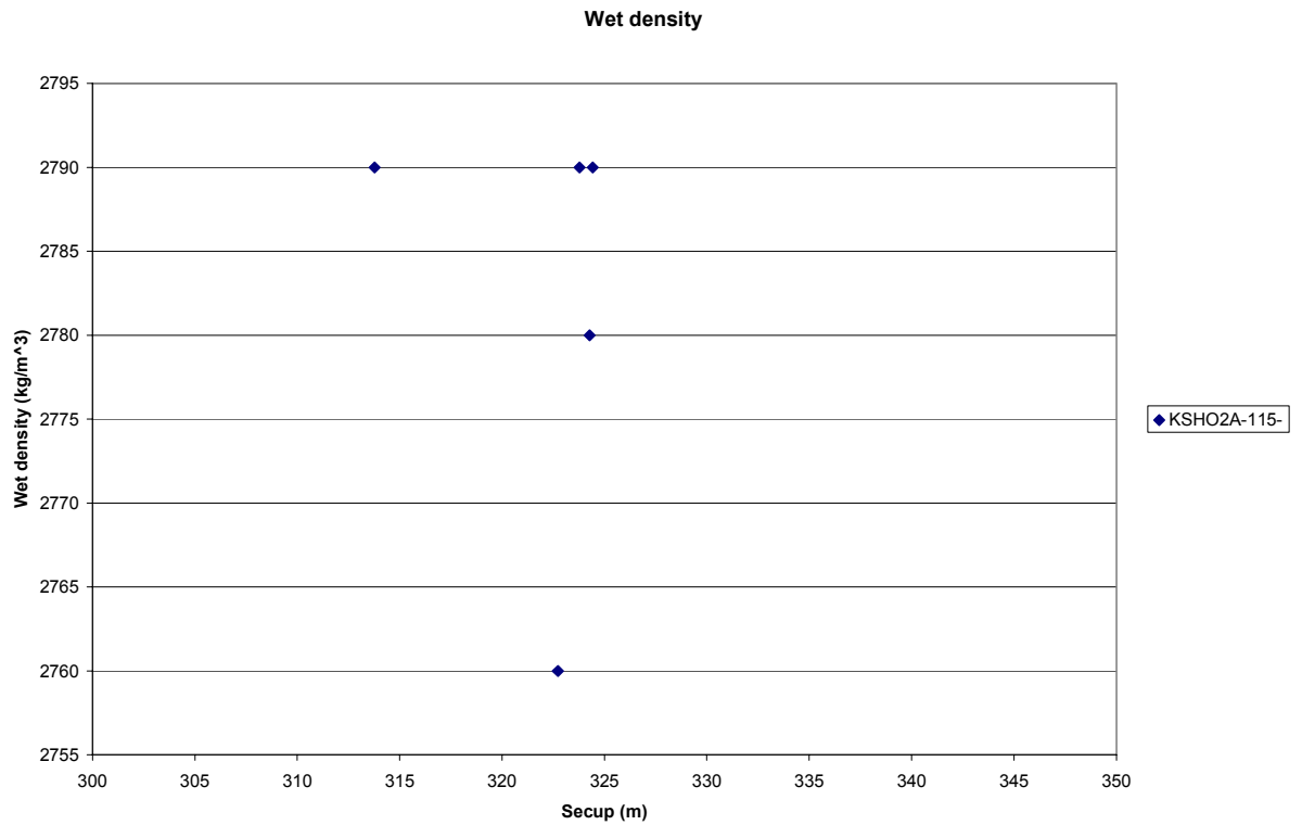
Figure 5-1. Density versus depth at which the samples are taken in the borehole.
