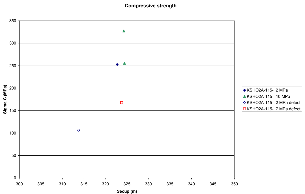
Figure 5-2. Compressive strength versus depth at which the samples are taken in the borehole.
