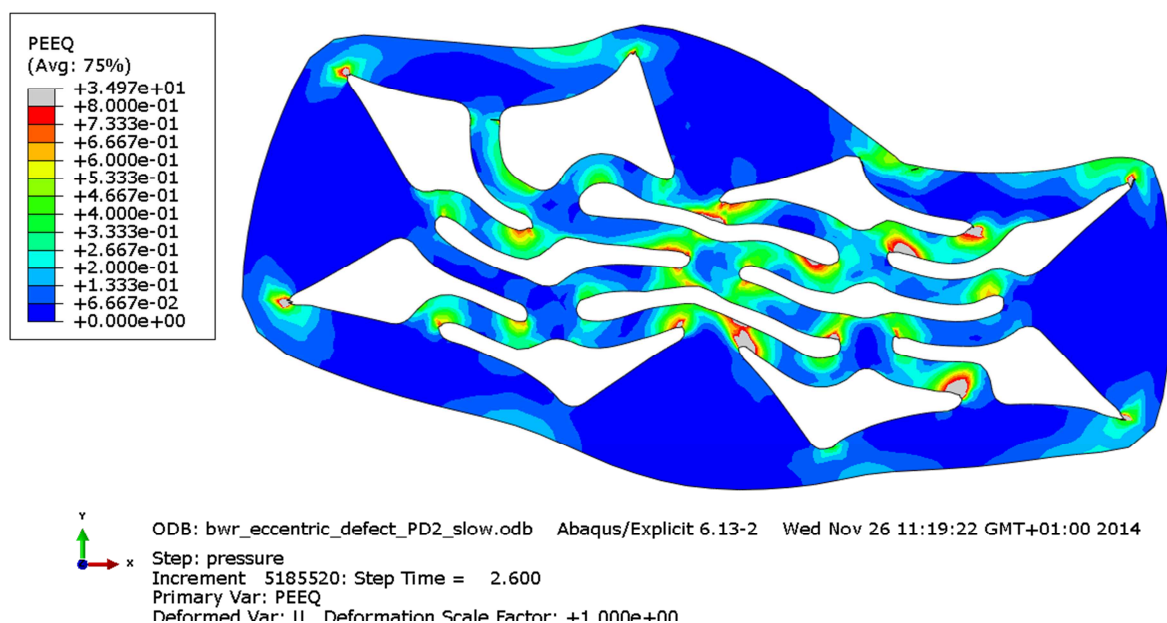
Figure 12-4. Displaced geometry with equivalent plastic strain (PEEQ) for case bwr_eccentric_defect_PD2 slow loading.
