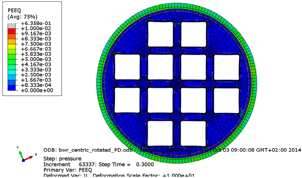
Figure A1-1 Equivalent plastic strain (PEEQ) with 60 MPa as applied hydrostatic pressure.
