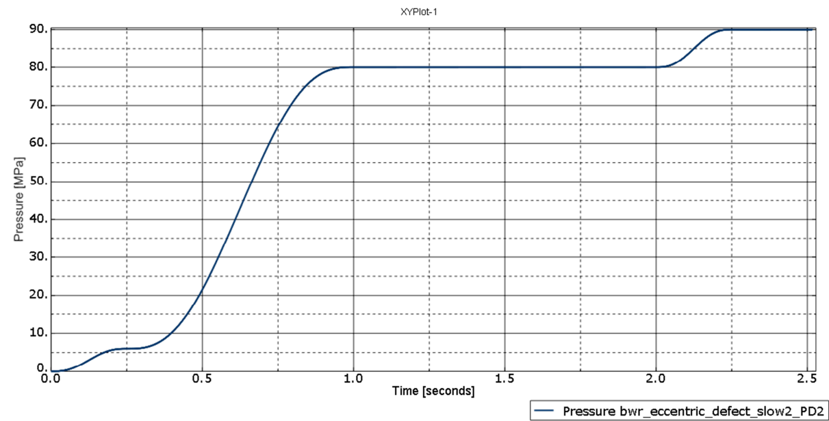
Figure 8-5. Hydrostatic pressure applied to the copper shell external surface for the BWR insert when the load is applied slowly and with constant load before the first expected instability to stabilize the solution.
