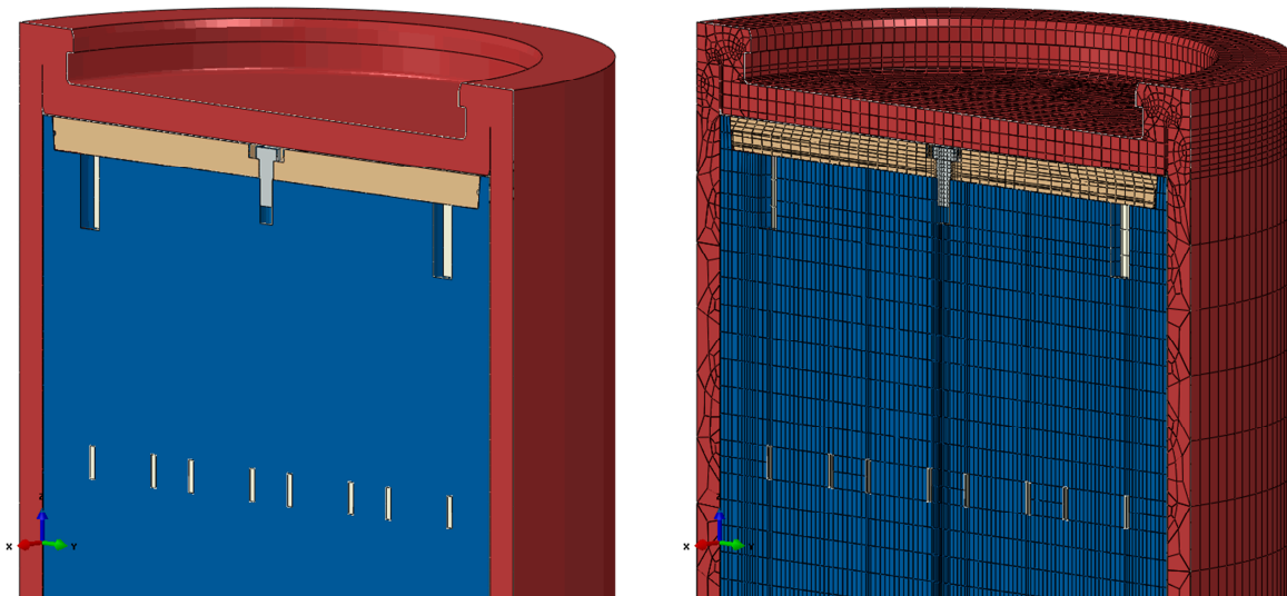
Figure 2-5. Details of the upper part of the BWR model, with the copper shell (red), insert lid (brown), insert (blue), channel tubes including support plates (white) and screw (grey).
