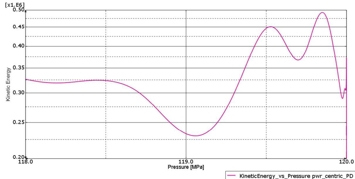
Figure 11-5. Kinetic energy versus pressure for the PWR insert for case pwr_centric_full_PD.
