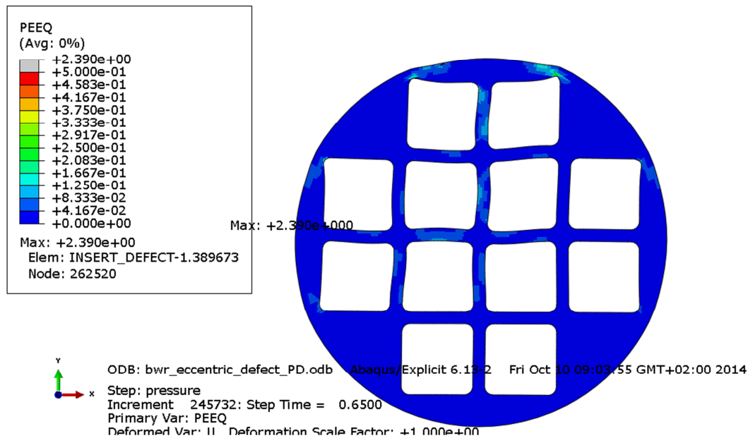
Figure A3-6 Equivalent plastic strain (PEEQ) for the insert with 120 MPa as applied hydrostatic pressure.
