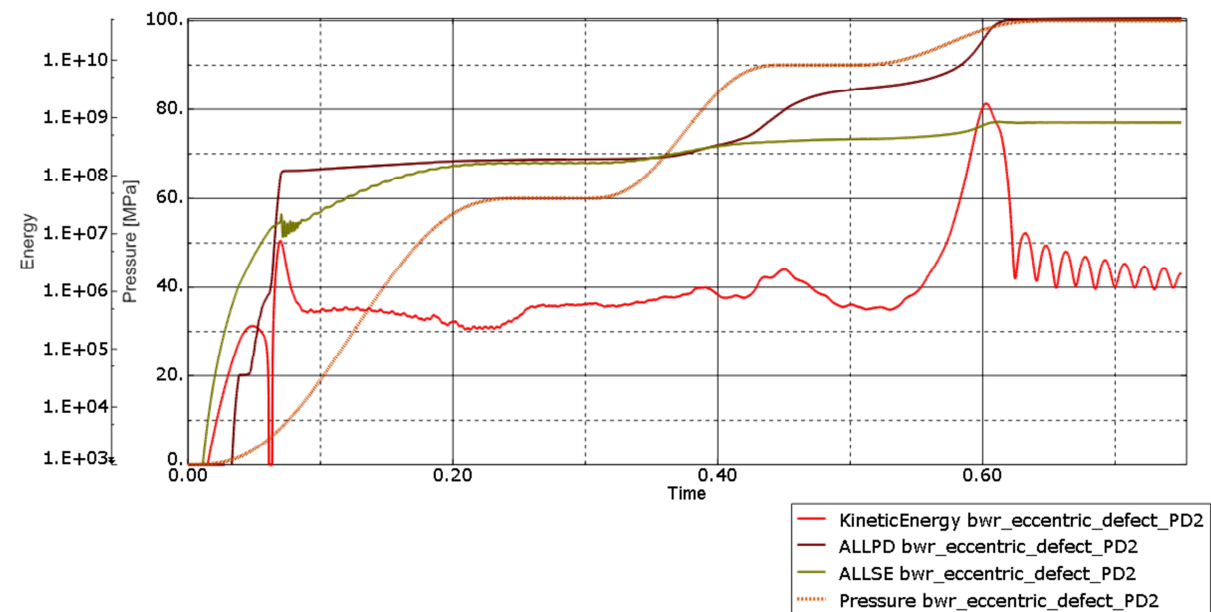
Figure 11-23. Kinetic and plastic energy together with pressure versus time [seconds] for the BWR insert for case bwr_eccentric_defect_PD2 .
