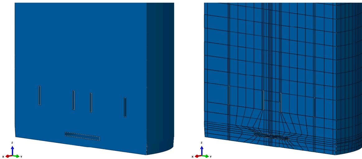
Figure 3-16. PWR insert, lower geometry (left) and mesh (right).
