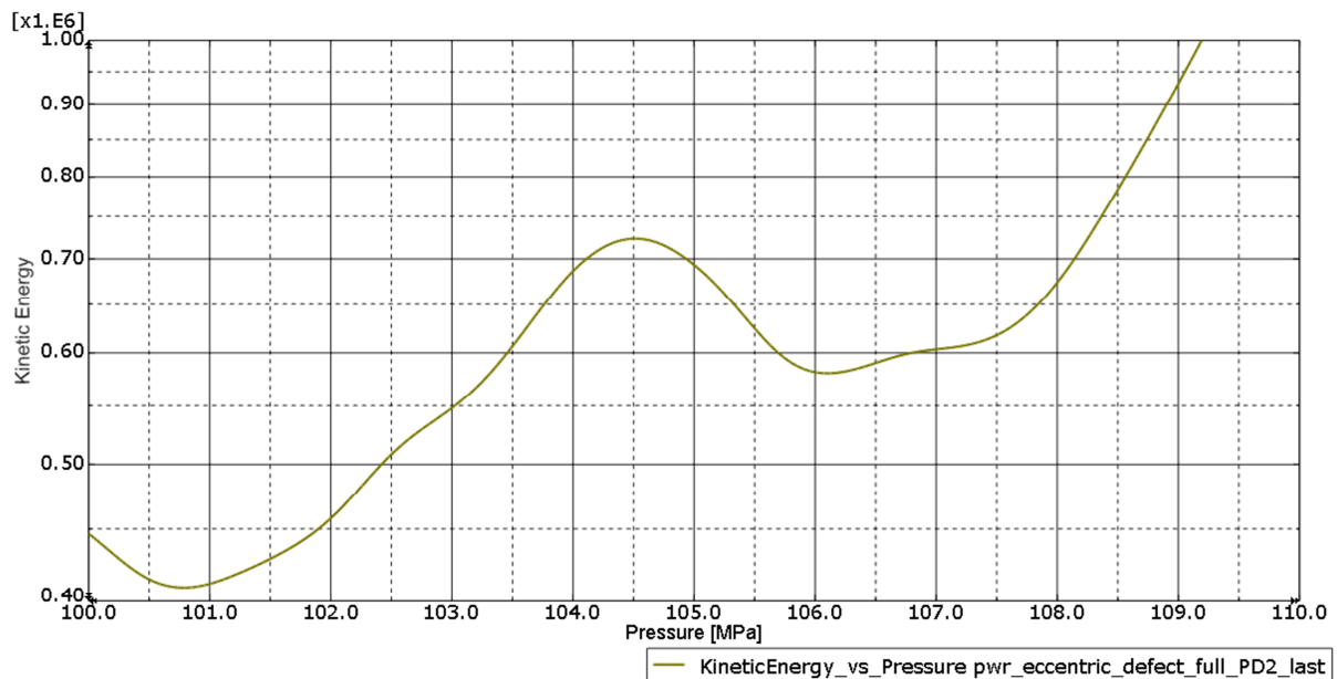
Figure 11-11. Kinetic energy versus pressure for the PWR insert for case pwr_eccentric_defect_full_PD2 .
