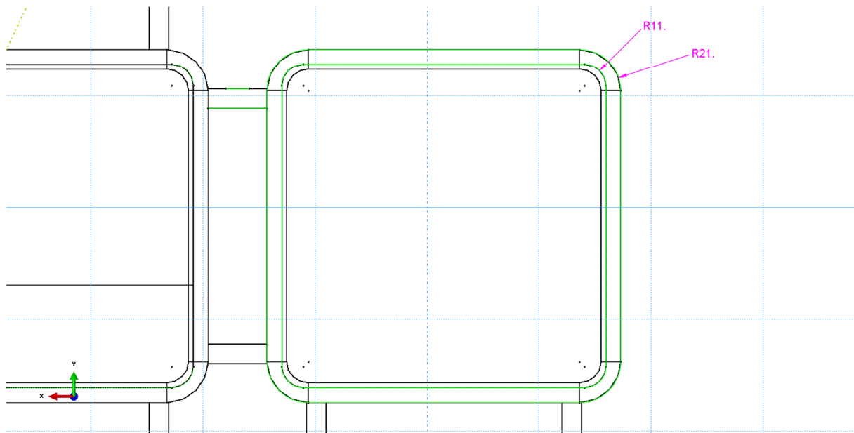
Figure 3-13. Plot that shows corner radius for the channel tubes. Also the modified geometry for the support plates with the weld is included. Also note that the inner weld string from manufacturing of welded tubes (shown at the CAD-drawing) has been removed.
