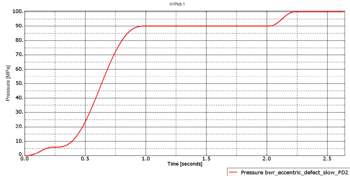
Figure 8-4. Hydrostatic pressure applied to the copper shell external surface for the BWR insert when the load is applied slowly.
