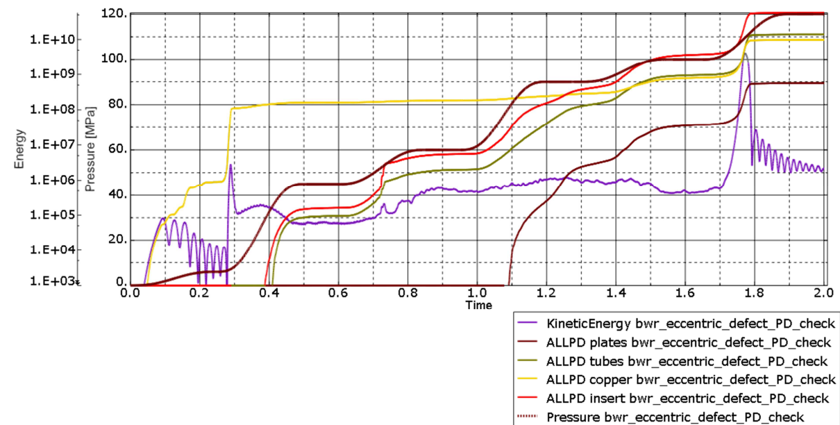
Figure 11-21. Kinetic and plastic energy together with pressure versus time [seconds] for the BWR insert for case bwr_eccentric_defect_PD.
