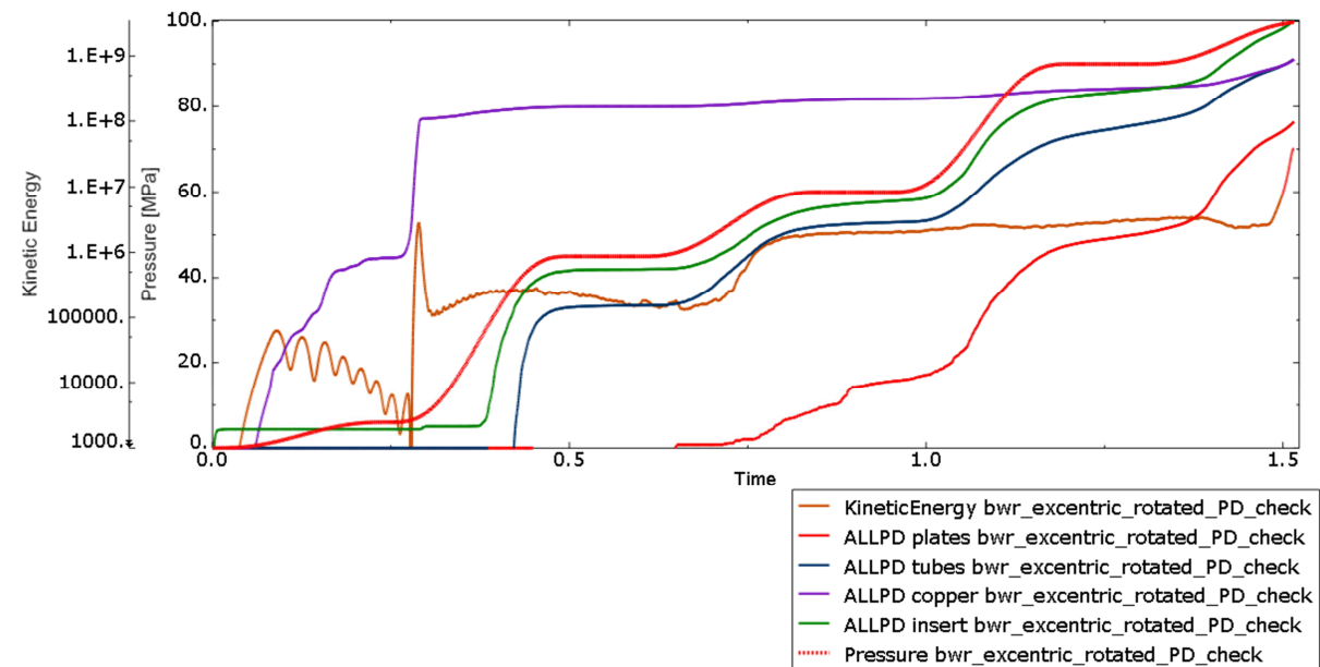
Figure 11-19. Kinetic and plastic energy together with the pressure versus time [seconds] for the BWR insert for case bwr_excentric_rotated_PD .
