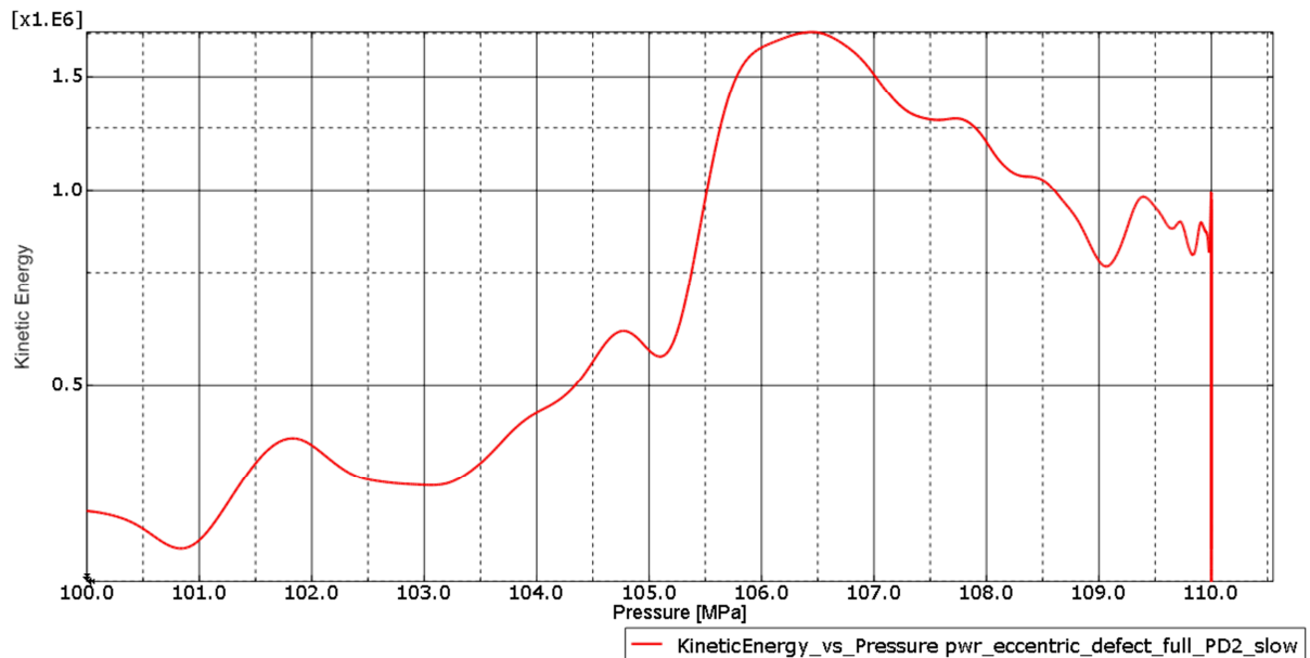
Figure 11-13. Kinetic energy versus pressure for the PWR insert for case pwr_eccentric_defect_full_PD2 – slow loading .
