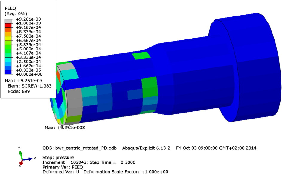
Figure A1-14 Equivalent plastic strain (PEEQ) for the fixing screw with 90 MPa as applied hydrostatic pressure.
