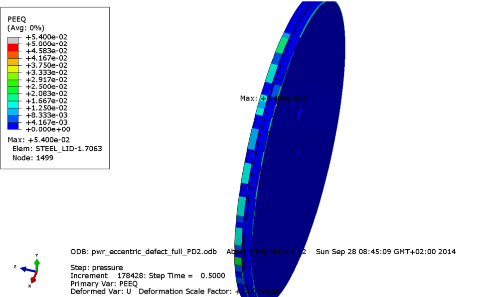
Figure A8-13 Equivalent plastic strain (PEEQ) for the insert lid with 90 MPa as applied hydrostatic pressure.
