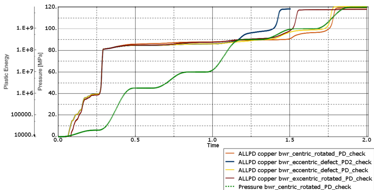
Figure 11-15. Plastic energy and pressure versus time [seconds] for the BWR insert.
