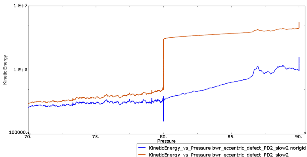
Figure 11-28. Kinetic energy versus pressure for the BWR insert for case bwr_eccentric_defect_PD2 – slow2 loading. Curve labelled “kinetic bwr_eccentric_defect_PD2_slow2 norigid” corresponds to when rigid body motion is removed.
