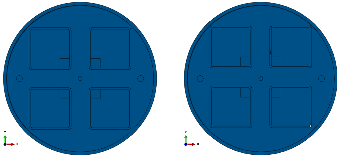
Figure 3-17. PWR insert with channel tubes symmetrically positioned (left) and eccentrically positioned (right) – top view.
