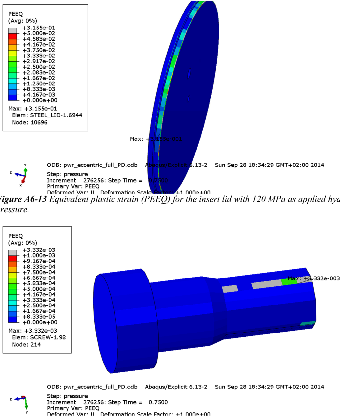
Figure A6-14 Equivalent plastic strain (PEEQ) for the fixing screw with 120 MPa as applied hydrostatic pressure.
