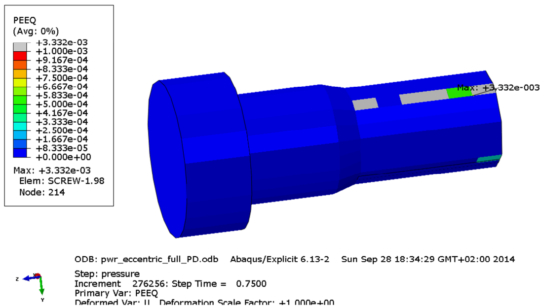
Figure A6-14 Equivalent plastic strain (PEEQ) for the fixing screw with 120 MPa as applied hydrostatic pressure.
