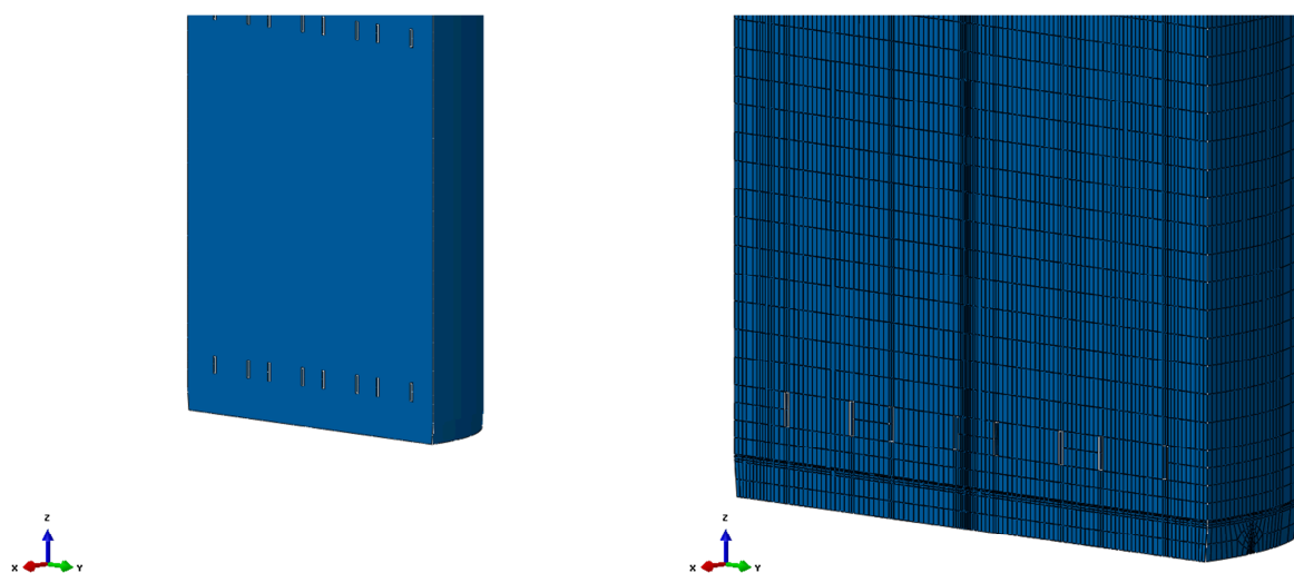
Figure 3-6. BWR insert, lower geometry (left) and mesh (right).
