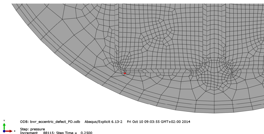
Figure 10-1. Example of bad elements creating unrealistically high stress and strain magnitudes (red colour).
