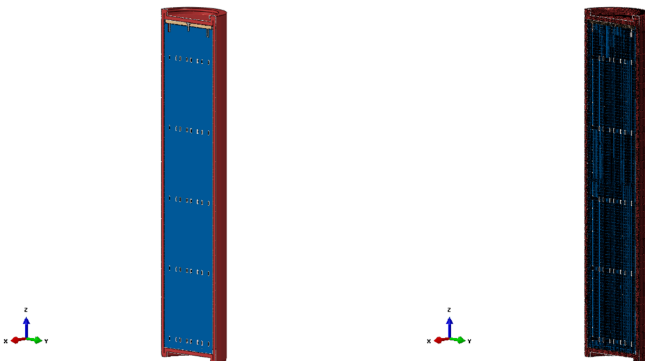
Figure 2-4. The BWR model (half of the model is shown), with the copper shell (red), insert lid (brown), insert (blue), channel tubes (white) and screw (grey).
