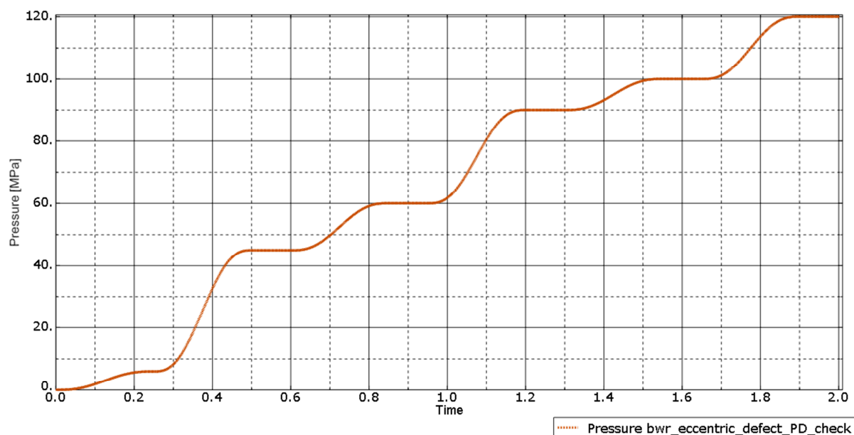
Figure 8-1. Hydrostatic pressure applied to the copper shell external surface for the BWR insert.
