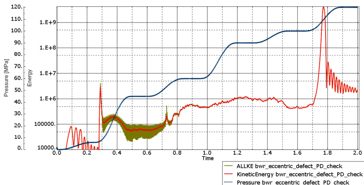
Figure 9-1. Example of filtering with cut-off at 100 Hz. The high frequency noise after initial contact between insert and copper shell at about 0.3 seconds disappears completely. Time scale in seconds.
