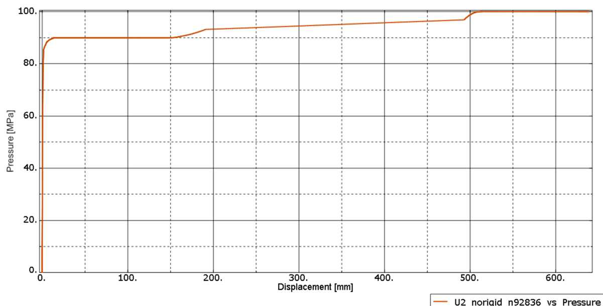
Figure 12-2. Displacement versus pressure for case bwr_eccentric_defect_PD2 slow loading.
