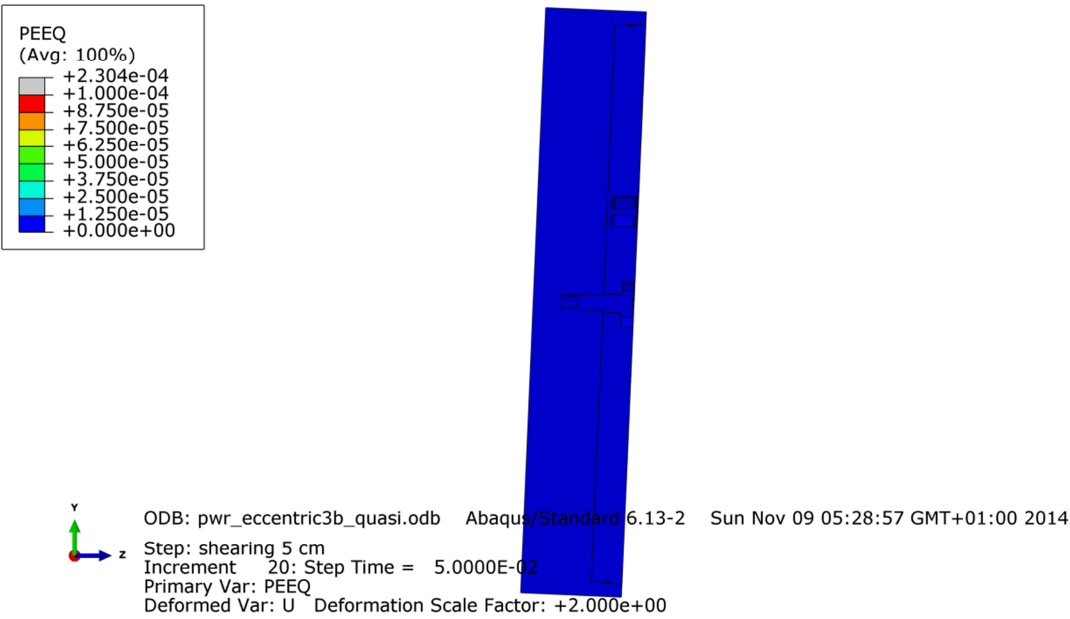
Figure A3-15. Plot shows equivalent plastic strain (PEEQ) close to the insert lid fixing screw after 5 cm shearing.
