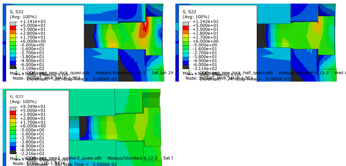
Figure 9-51. Plots show lateral stress (S22) in the screw after 5 cm shearing. Upper left shows shearing at the lid using initial stress 355 MPa, top right shows shearing at the lid using initial stress 177.5 MPa and lower left shows shearing at 3/4-distance from the insert base when screw stress is specified to 81 MPa.
