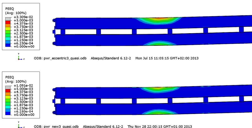
Figure 9-27. Plots show equivalent plastic strain (PEEQ) for the steel channel tubes after 6 cm shearing for eccentric PWR model (upper) and the centric PWR model (lower).
