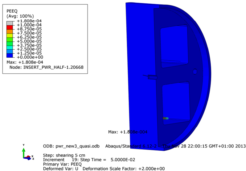
Figure A1-8. Plot shows equivalent plastic strain (PEEQ) for the insert top after 5 cm shearing.
