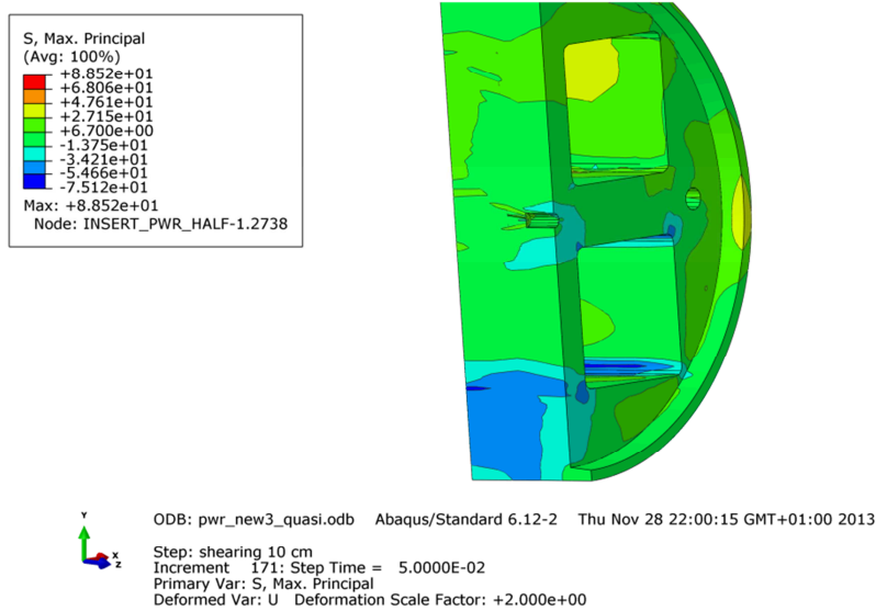
Figure 9-45. Plot shows maximum principal stress [MPa] for the insert top after 10 cm shearing at 3/4-distance from the insert base.
