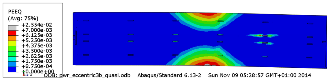
Figure 9-33. Plots show plastic equivalent strain (PEEQ) for the insert after 6 cm shearing for eccentric PWR model with compressive stress at the thinnest region (upper) and with tensile stress at the thinnest region (lower).
