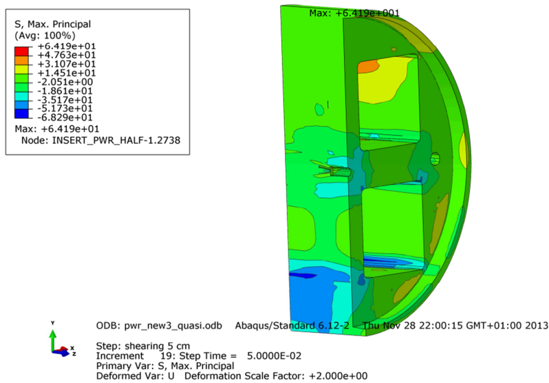
Figure A1-7. Plot shows maximum principal stress [MPa] for the insert top after 5 cm shearing.
