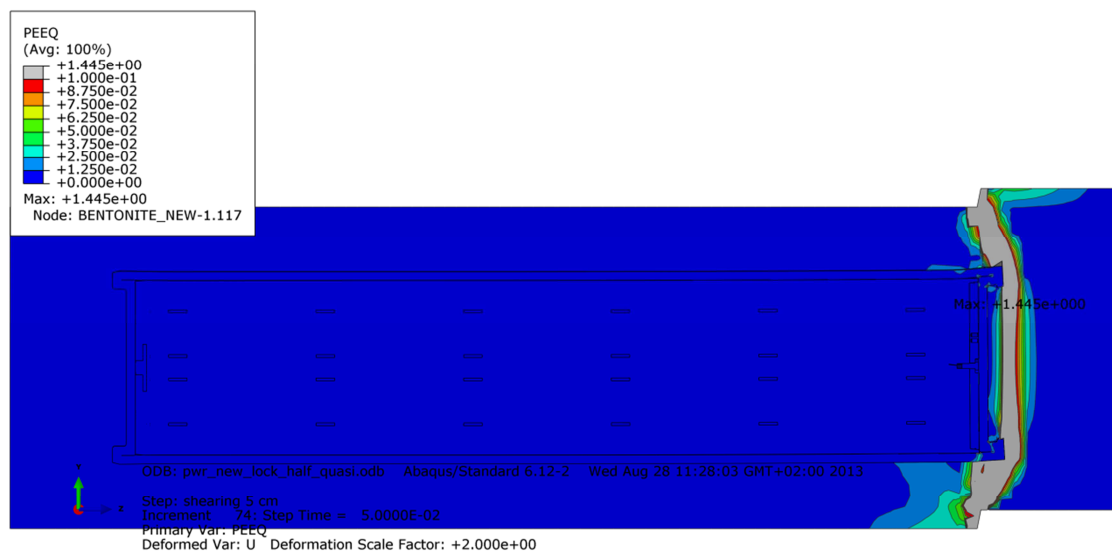
Figure A6-1. Plot shows equivalent plastic strain (PEEQ) after 5 cm shearing.
