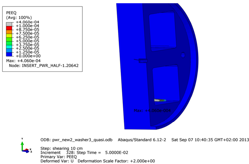
Figure A7-23. Plot shows equivalent plastic strain (PEEQ) for the insert top after 10 cm shearing.
