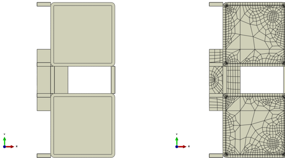
Figure 3-9. Steel channel tubes geometry (left), and mesh (right) – bottom view showing also the support plates.
