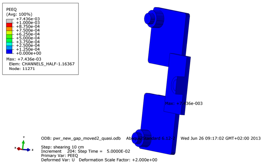
Figure A4-27. Plot shows equivalent plastic strain (PEEQ) for the steel channel tubes base plates after 10 cm shearing.
