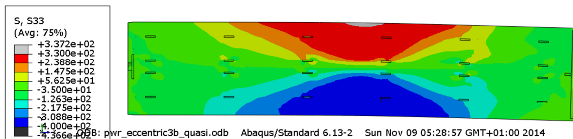
Figure 9-32. Plots show axial stress [MPa] for the insert after 6 cm shearing for eccentric PWR model with compressive stress at the thinnest region (upper) and with tensile stress at the thinnest region (lower).
