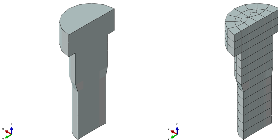
Figure 3-12. Screw geometry (left), and mesh (right) – used to fix the insert lid to the insert.
