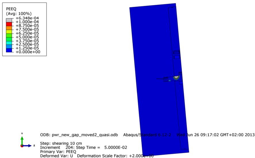
Figure A4-30. Plot shows equivalent plastic strain (PEEQ) close to the insert lid fixing screw after 10 cm shearing.
