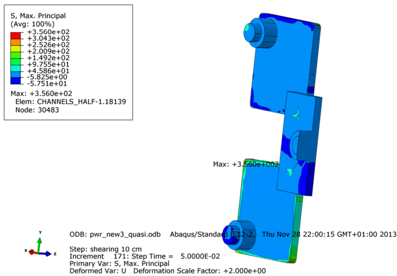
Figure 9-46. Plot shows maximum principal stress [MPa] for the steel channel tube plates at the base after 10 cm shearing at 3/4-distance from the insert base.
