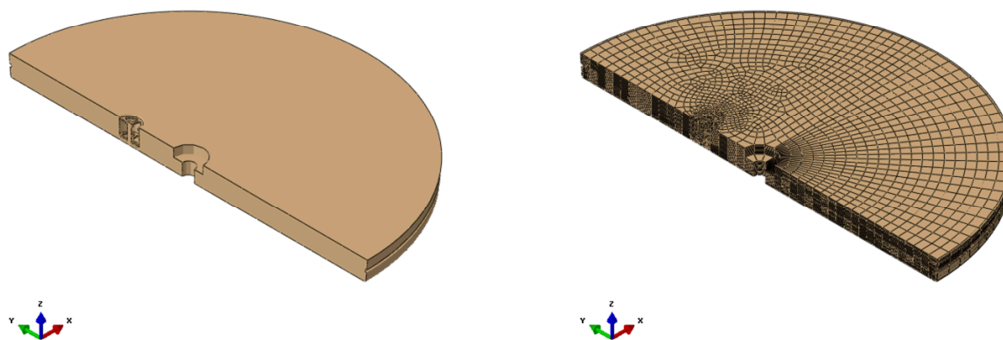
Figure 3-10. Insert lid geometry (left) and mesh (right).
