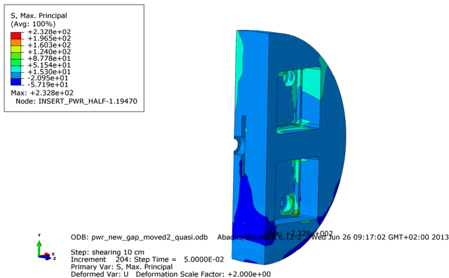
Figure A4-20. Plot shows maximum principal stress [MPa] for the insert base after 10 cm shearing.
