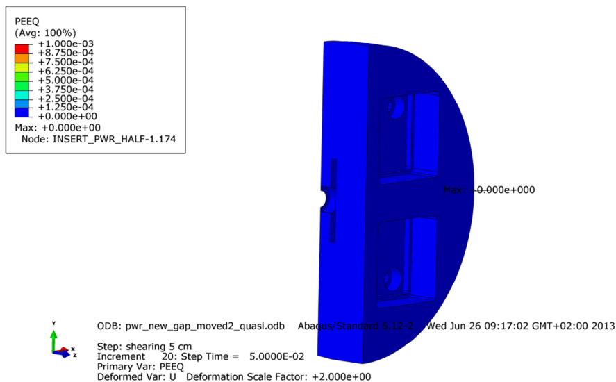
Figure A4-6. Plot shows equivalent plastic strain (PEEQ) for the insert base after 5 cm shearing.
