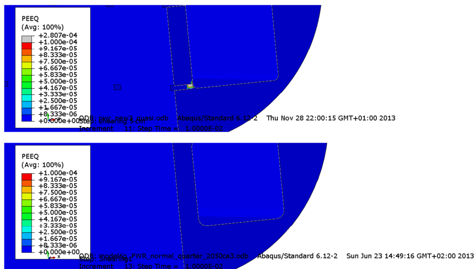
Figure A8-10. Plot shows plastic equivalent strain (PEEQ) for the insert after 5 cm shearing for detailed PWR model (upper) and the reference PWR model (lower).
