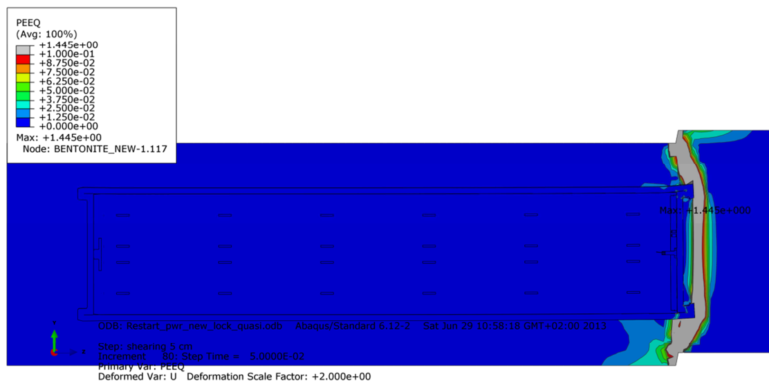
Figure A5-1. Plot shows equivalent plastic strain (PEEQ) after 5 cm shearing.
