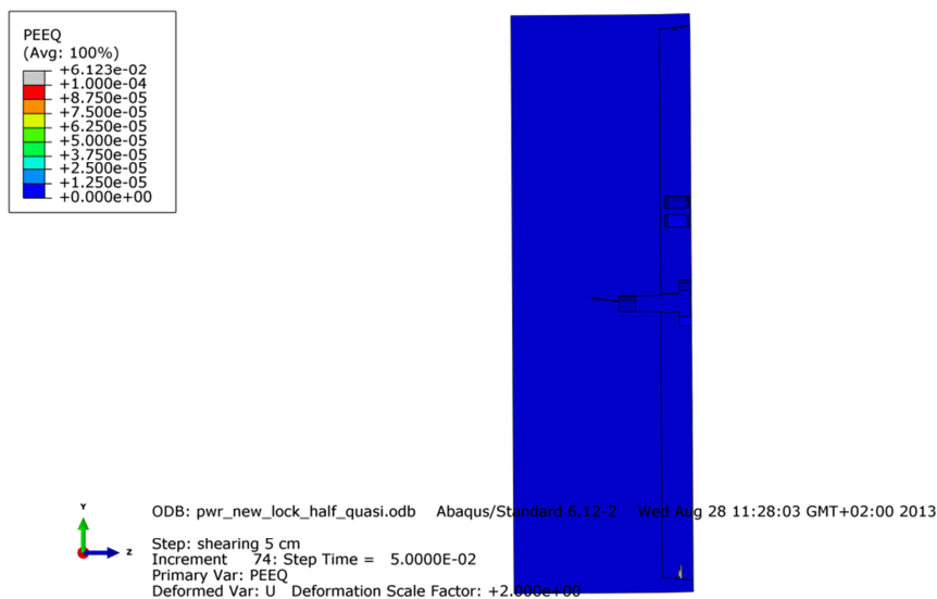
Figure A6-15. Plot shows equivalent plastic strain (PEEQ) close to the insert lid fixing screw after 5 cm shearing.
