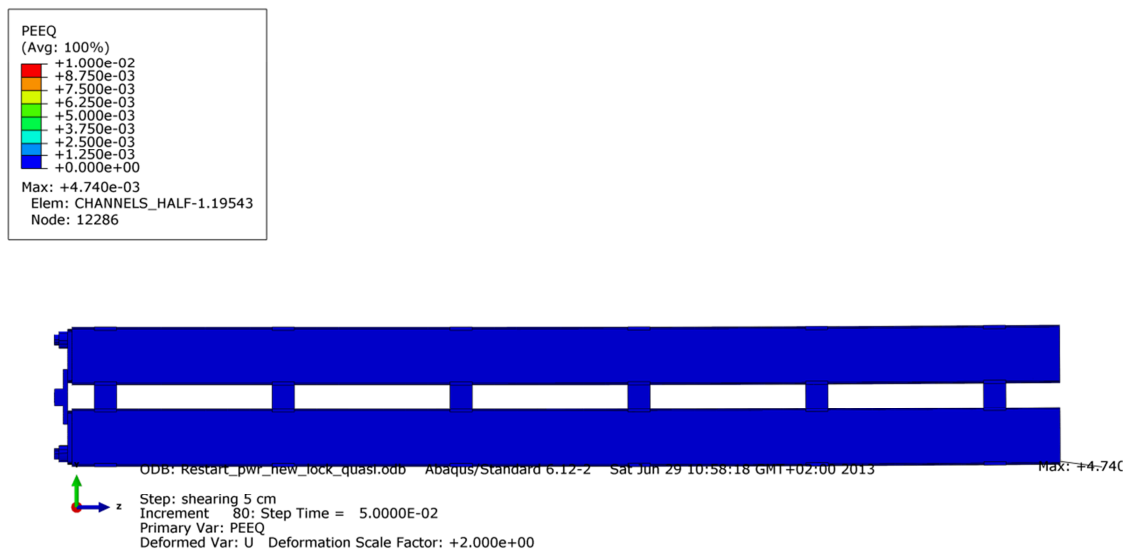
Figure A5-10. Plot shows equivalent plastic strain (PEEQ) for the steel channel tubes after 5 cm shearing.
