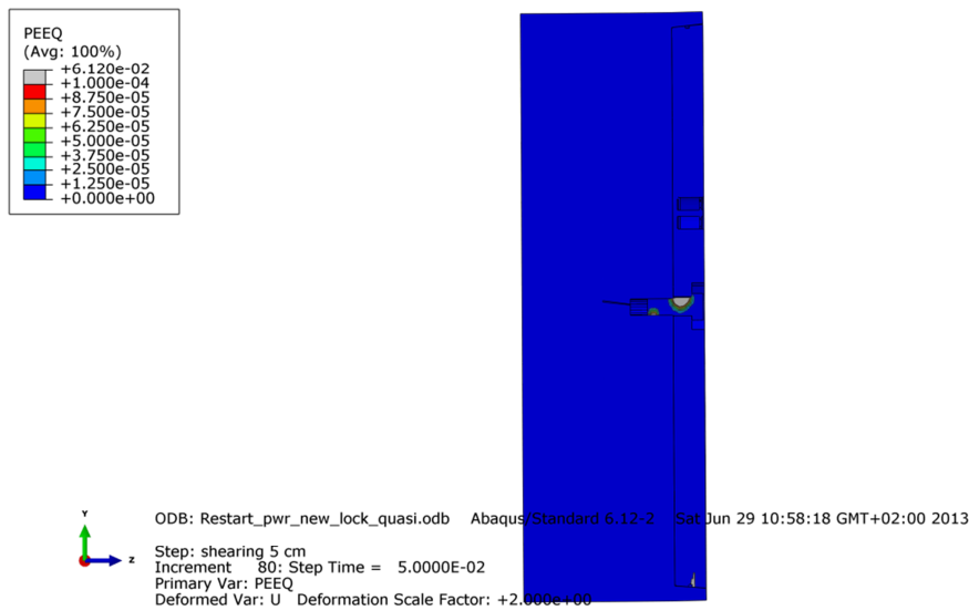
Figure A5-15. Plot shows equivalent plastic strain (PEEQ) close to the insert lid fixing screw after 5 cm shearing.
