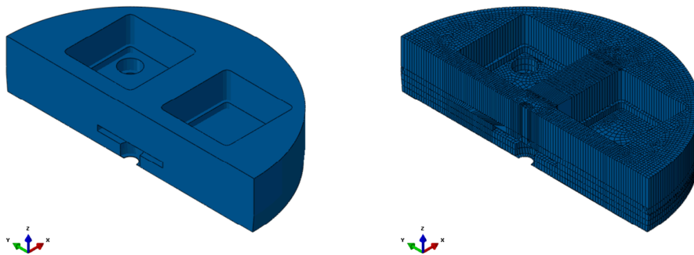
Figure 3-5. Insert PWR geometry (left), and mesh (right) – base plate.
