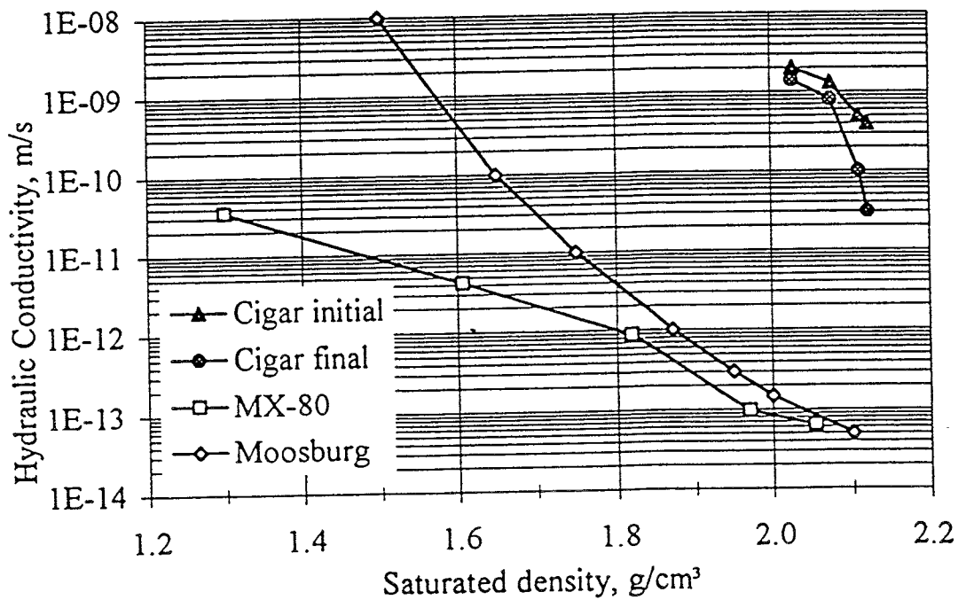
Figure 4.6: Hydraulic conductivity of the Cigar Lake material and two commercial bentonites versus clay density at saturation.
