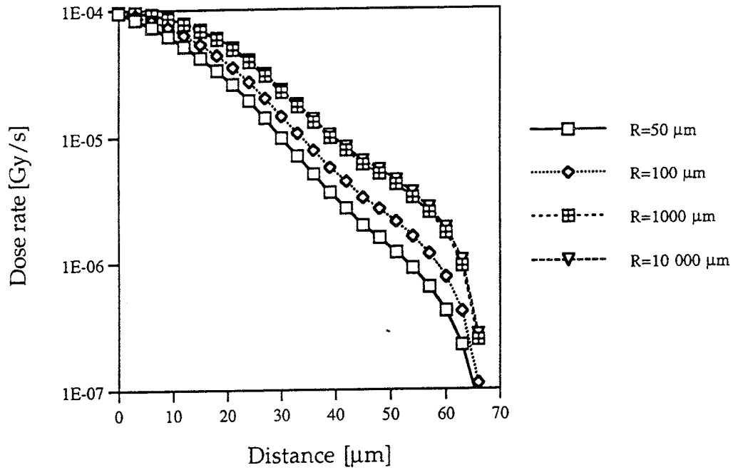
Figure 4.1: Alpha dose rates at varying distances and radii (R) for an absorber with density 1 \text{ kg/dm}^3
