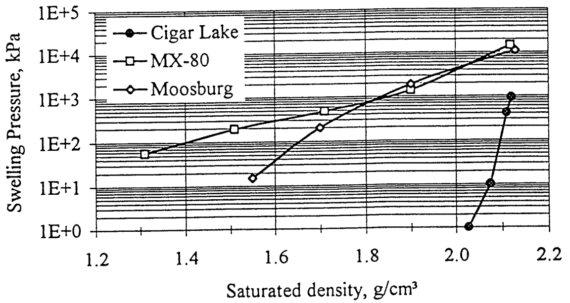
Figure 4.5: Swelling pressure of the Cigar Lake material and two commercial bentonites versus saturated clay density. MX-80 represents a natural sodium bentonite and Moosburg a natural calcium bentonite.
