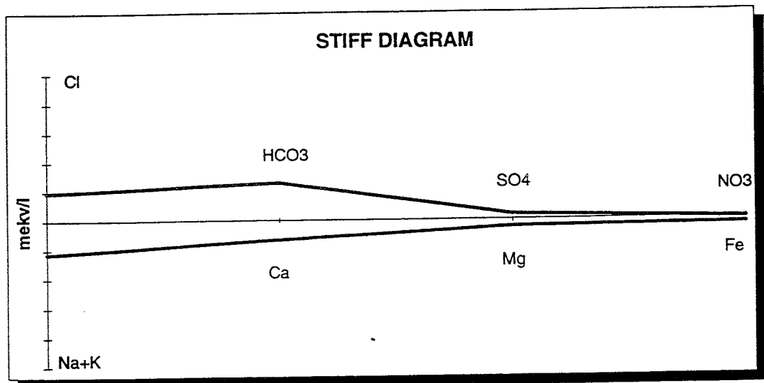
Figure 5.4: Example of a Stiff diagram, calculated from one of the reference groundwater compositions
