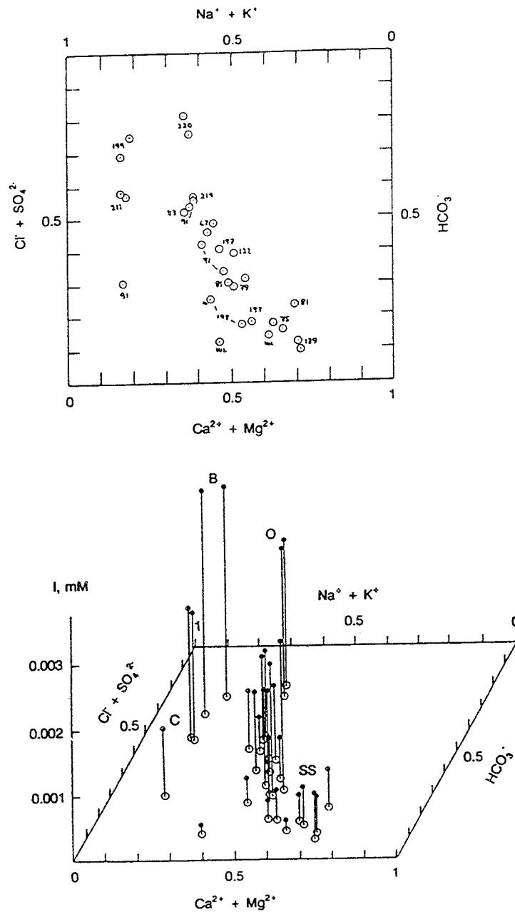
Figure 5.3: Piper Plot of the major components in the sampled groundwaters (B = basement; O = ore; SS = sandstone)
